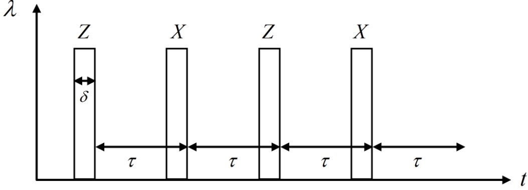
FIG. 4. Schematic of the pulse sequence used to suppress general single-qubit decoherence. This pulse sequence is sometimes called XY-4, or the universal decoupling sequence.
