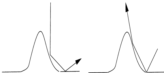
Fig. 1. On the left, the first collision strikes the adsorbate, the second strikes the surface. The reverse sequence occurs on the right.
