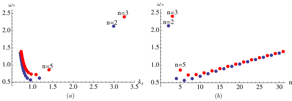
Figure 2. The second class of peaks for a specific value of magnetic field set by H = -0.1 . (a) The dependence on Fermi momentum. (b) The dependence on the Landau level number.
