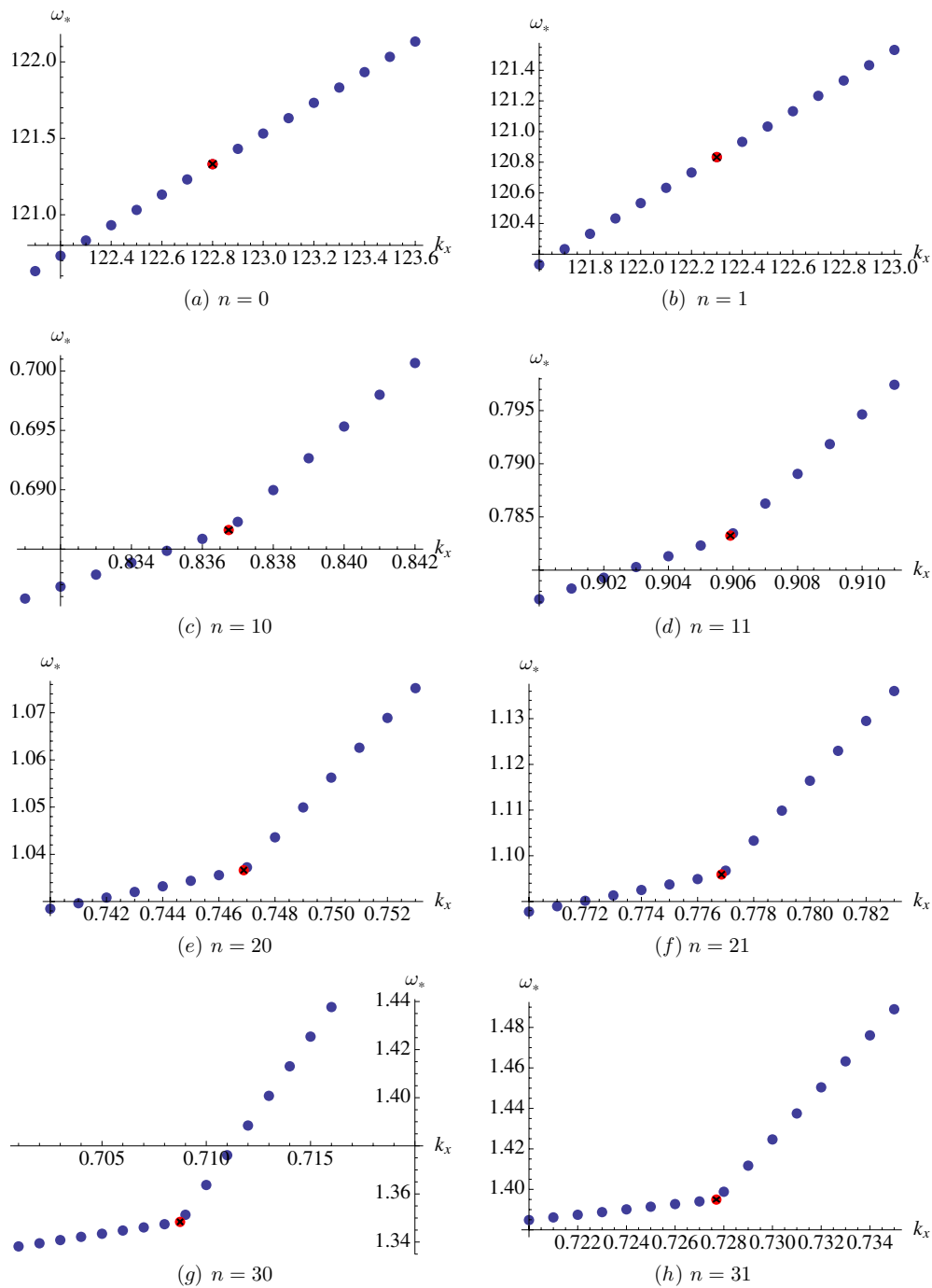
Figure 4. Dispersion behavior near the pole. The red dot marked with a cross marks the position of the pole.
