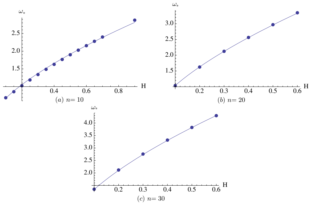
Figure 3. Behavior with increasing H for the poles in the regular regime. The best-fit line is given in equation (79).
