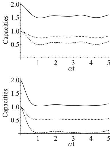
FIG. 2. Capacities C_E = 1 + Q (solid), Q_E = C_E/2 (dotted), and Q (dashed) as a function of dimensionless time \alpha t , of a qubit coupled to an Ising spin bath with N = 4 , for random values of g_n and \Omega_n . (Top) \beta = 10 ; (bottom) \beta = 1 . See text for additional details.
