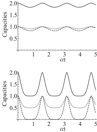
FIG. 4. Capacities C_E (solid), Q_E (dotted), and Q (dashed) as a function of dimensionless time \alpha t , of a qubit coupled to an Ising spin bath with N = 4 , for g_n = 1 and \Omega_n = 1 \forall n . (Top) \beta = 5 ; (bottom) \beta = 1 .
