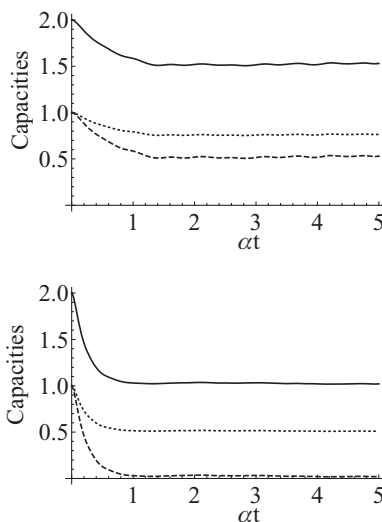
FIG. 3. Same as Fig. 2, with N = 100 .
