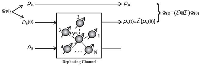
FIG. 1. Communication protocol: a qubit passes through an Ising spin-star channel. This is repeated in parallel over many such identical channels.
