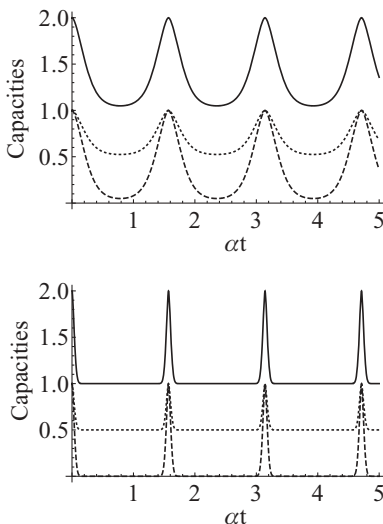
FIG. 5. Same as Fig. 4, with N = 100 .
